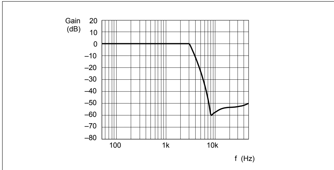
LPF Frequency Characteristics ( f_{\text{samp}} = 8.0 kHz)
