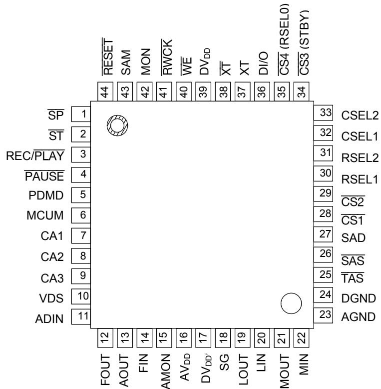
44-Pin Plastic QFP 44-Pin Plastic TQFP
