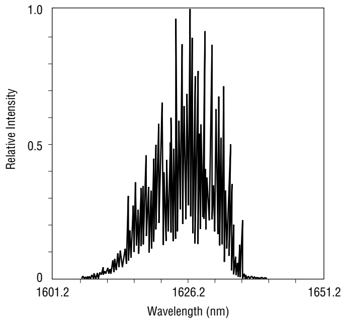
Oscillation Spectrum (T a =25°C)
