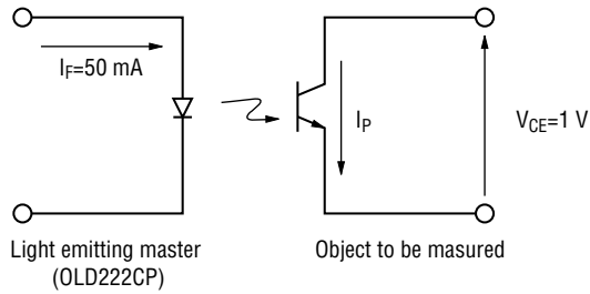
Measuring circuit
