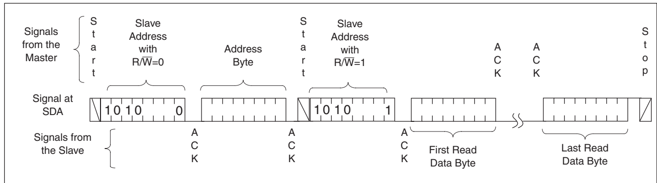
Figure 22. Read Sequence
