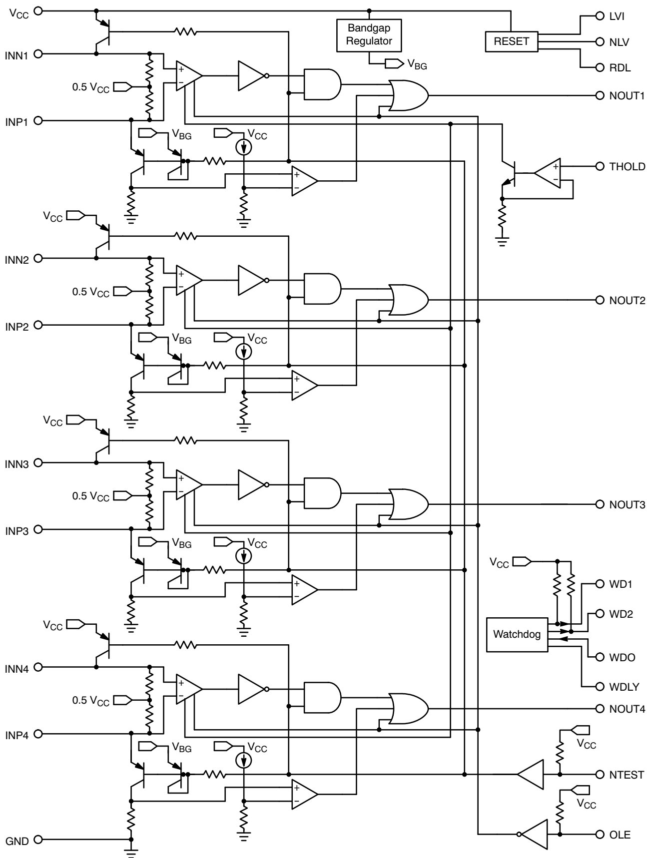
Figure 2. Block Diagram
