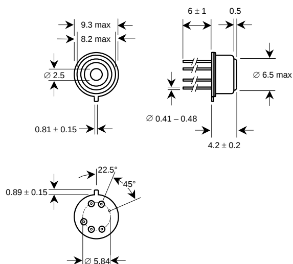
TO39 with high cap and int. reflector (C6 IRA): A1TPMI 336 IRA
