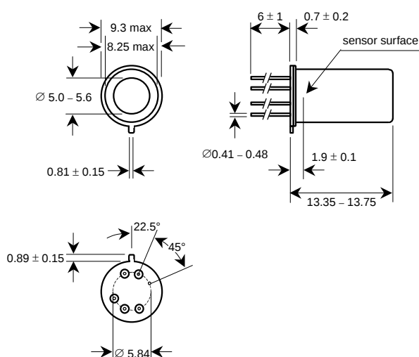
TO39 with high cap and int. reflector (C6 IRA): A1TPMI 336 IRA
