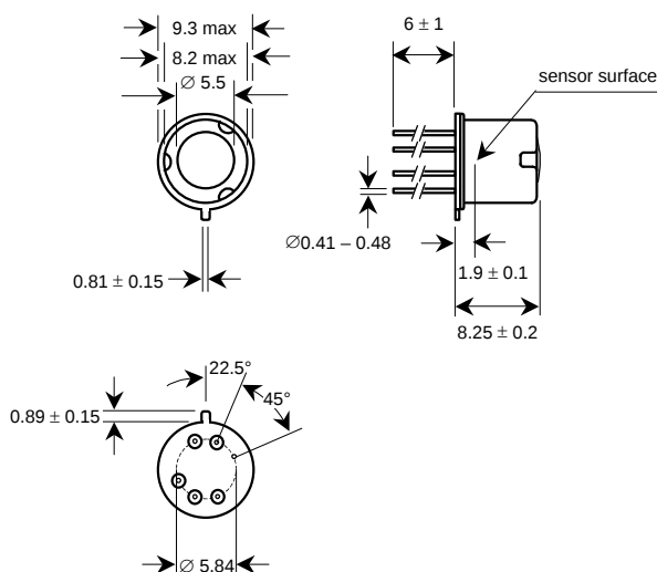
TO39 with low cap and square hole (C7) A1TPMI 337
