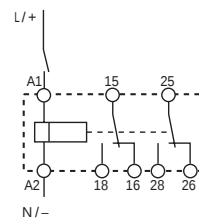
wiring diagram (without signal START)
