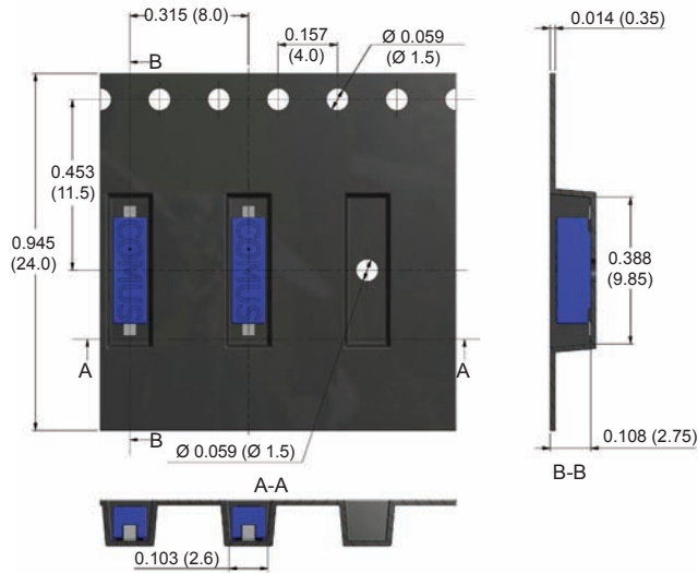
Dimensions for RI-80 SMDH G2 Tape and Reel All Dimension in inches (mm) nominal
