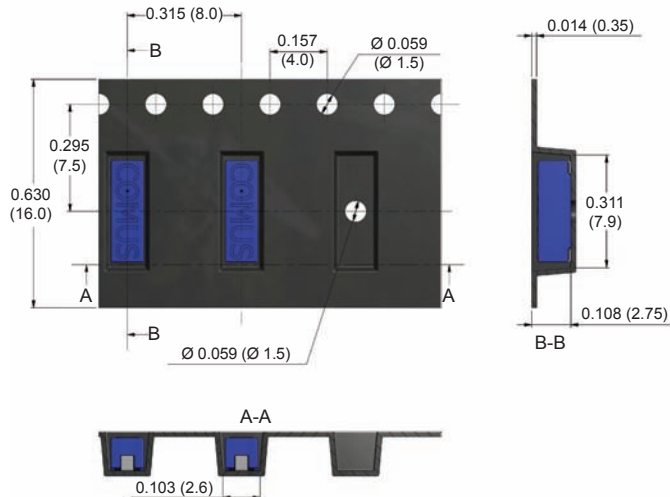
Dimensions for RI-80 SMDH J-Lead Tape and Reel All Dimension in inches (mm) nominal
