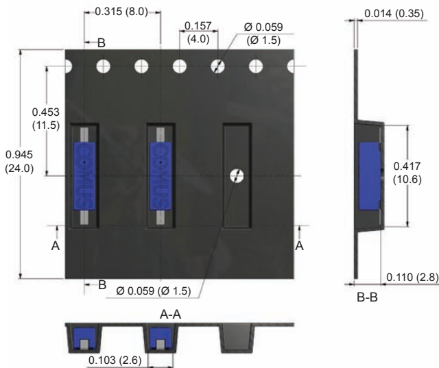
Dimensions for RI-80 SMDH J-Lead Tape and Reel All Dimension in inches (mm) nominal
