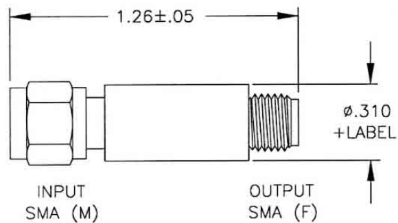
OUTLINE C
