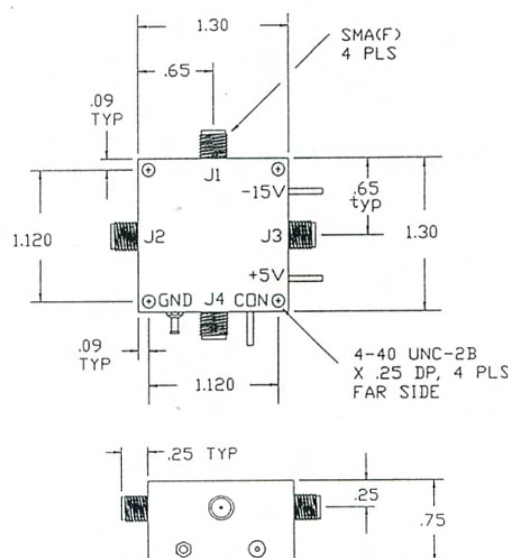
OUTLINE
