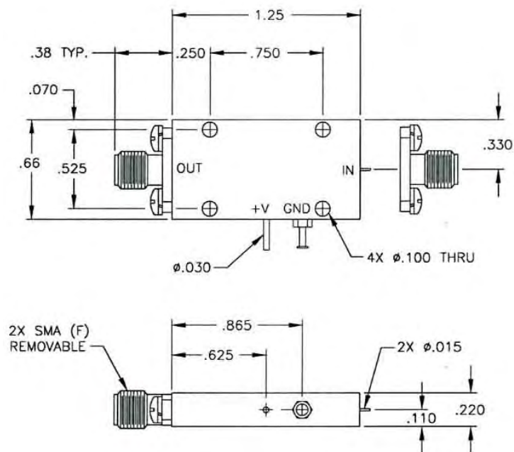
OUTLINE 3B
