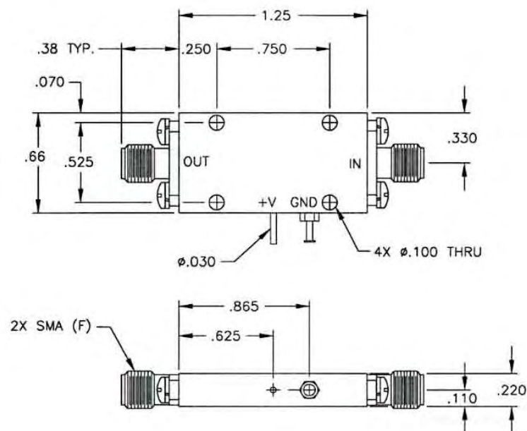
OUTLINE 3A
