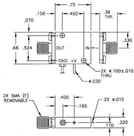
OUTLINE 1D
