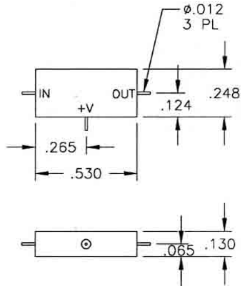
OUTLINE L3
