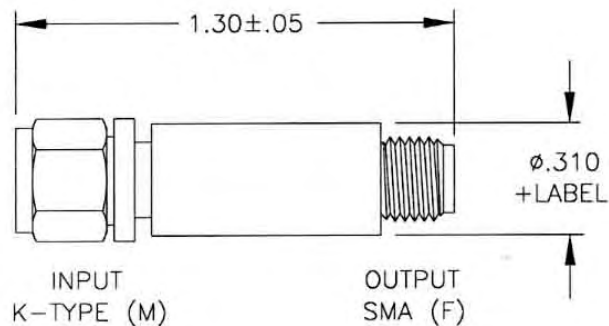
OUTLINE C1
