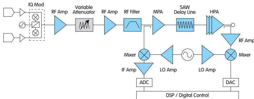
Base Station Transmitter &amp; PA
