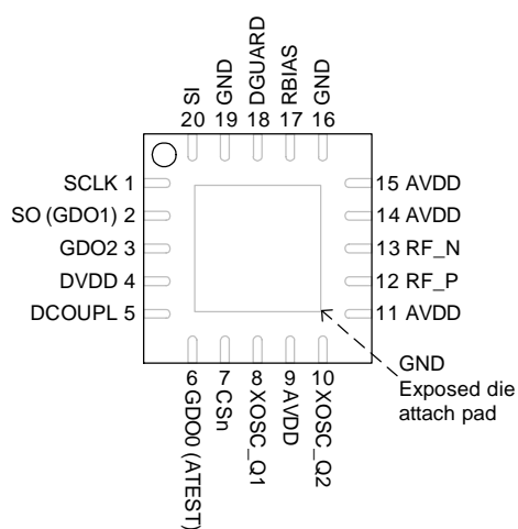
Figure 1: Pinout Top View
