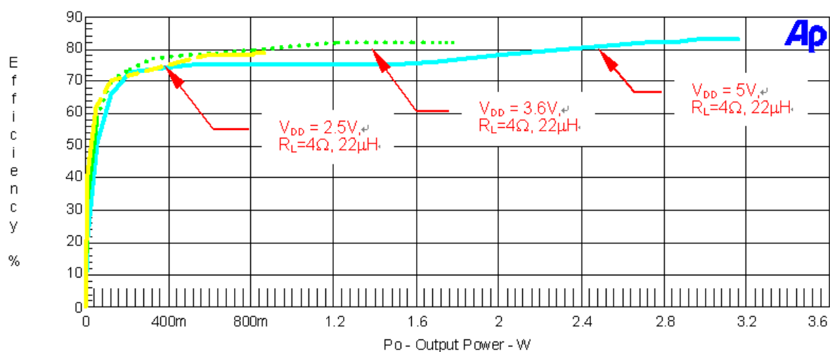
Figure 3. Efficiency vs. Output Power at 4Ω Load
