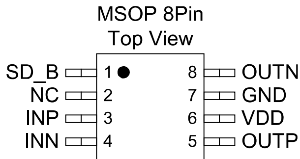
BA16852 MSOP 8Pin Top View
