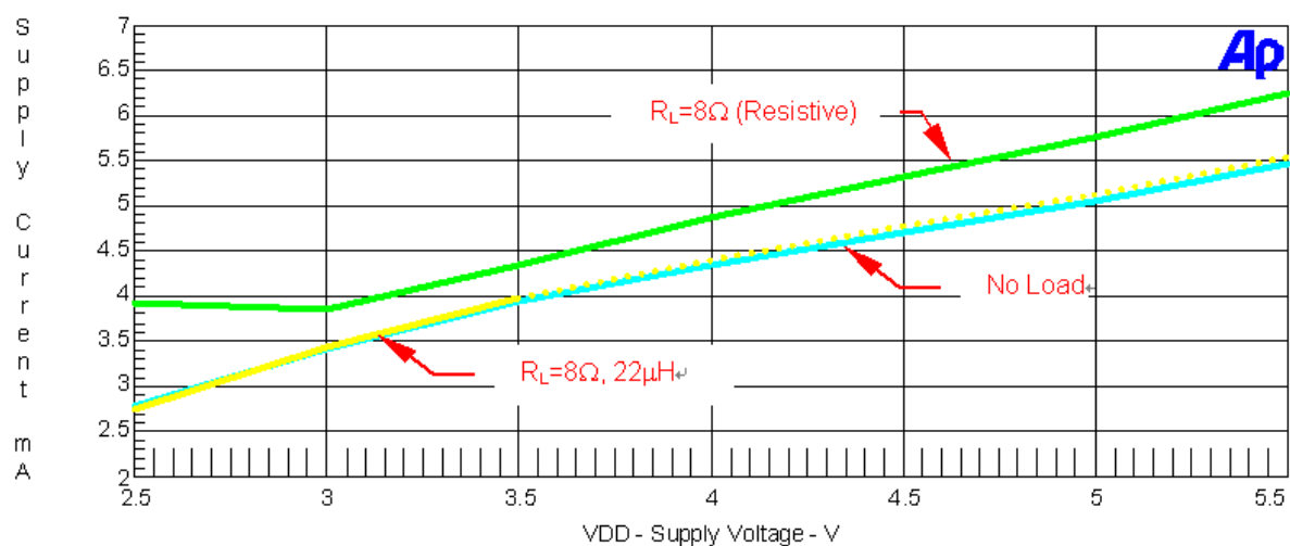
Figure 8. Quiescent Current vs. Supply Voltage
