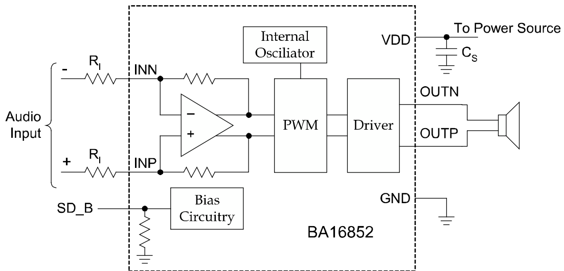
Figure 1. Typical BA16852 / BA16853 Application Circuit
