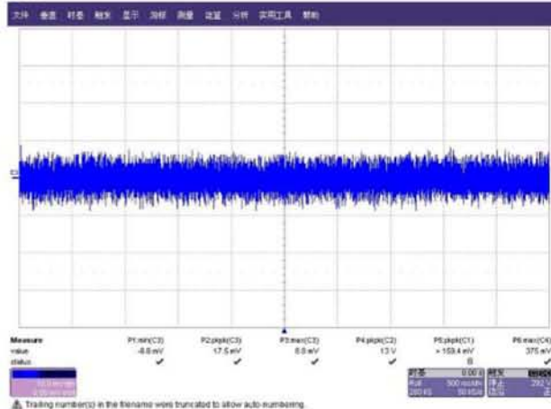
Figure 4: Measured ripple& noise waveform@264Vac/50HZ, full load
