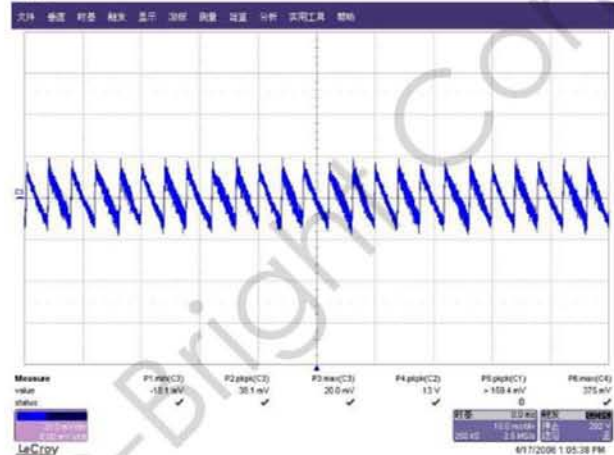
Figure 3: Measured ripple& noise waveform@264Vac/50HZ, no load
