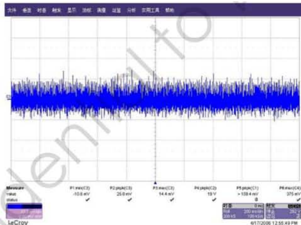
Figure 2: Measured ripple& noise waveform@90Vac/60HZ, full load
