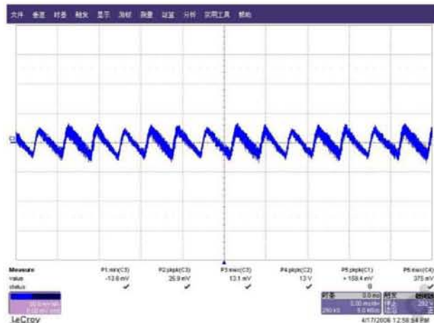
Figure 1: Measured ripple& noise waveform@90Vac/60HZ, no load
