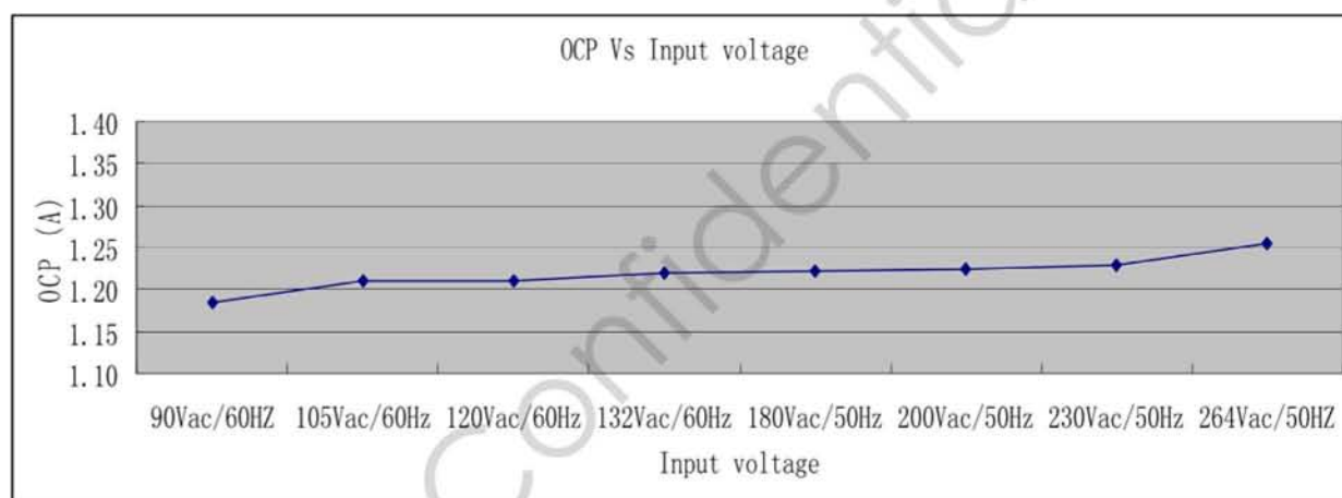
OCP curve
