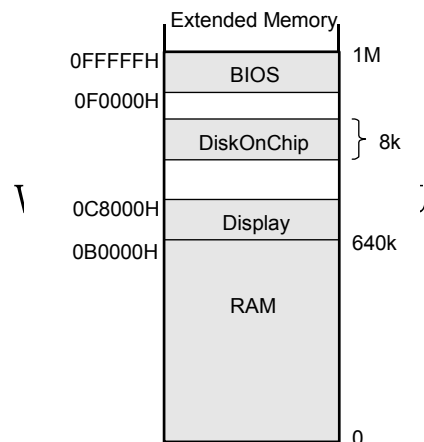
Figure 6: DiskOnChip 2000 Memory Window in the PC Memory Map
