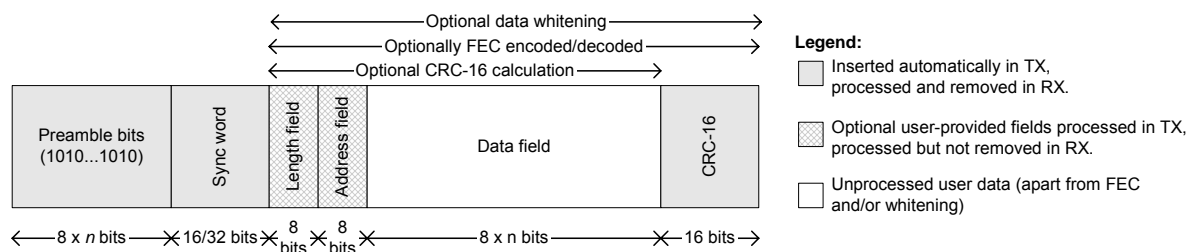
Figure 17: Packet Format
