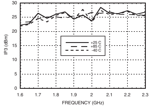
Single Channel: Input IP3 vs. Temperature
