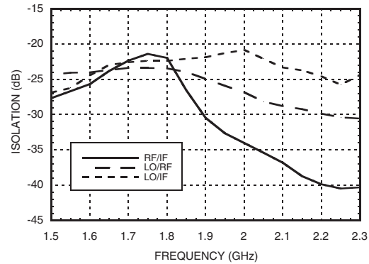
Single Channel: Isolation
