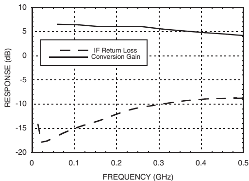
Single Channel: IF Bandwidth
