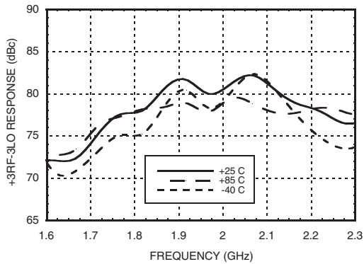
+3RF -3LO Response vs. Temperature [3]
