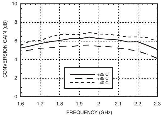
Single Channel: Conversion Gain vs. Temperature
