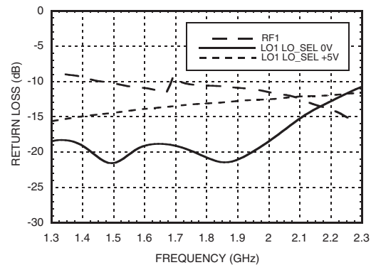
Single Channel: Return Loss
