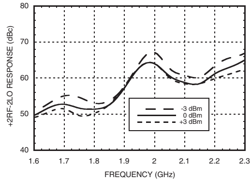
+2RF -2LO Response vs. LO Drive [3]
