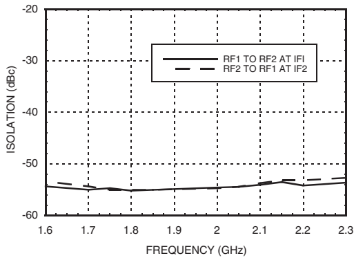
Dual Channel: Channel to Channel Isolation [1]
