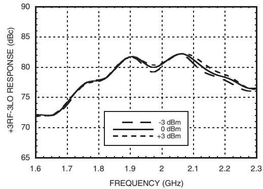
+3RF -3LO Response vs. LO Drive [3]
