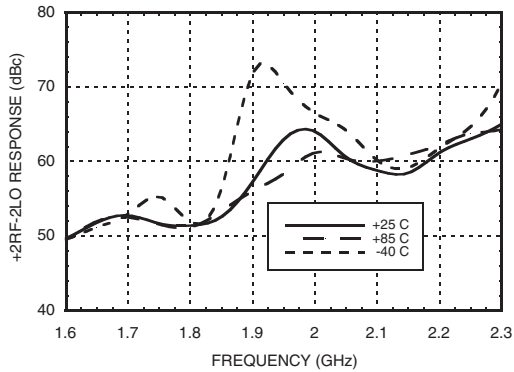
+2RF -2LO Response vs. Temperature [3]
