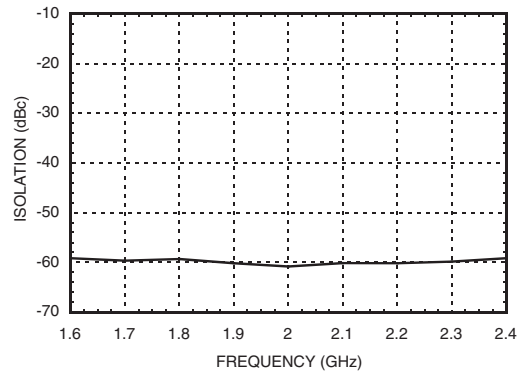
Dual Channel: LO1 to LO2 Isolation [2]
