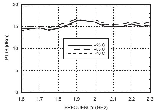
Single Channel: Input P1dB vs. Temperature
