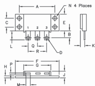
TO-249
