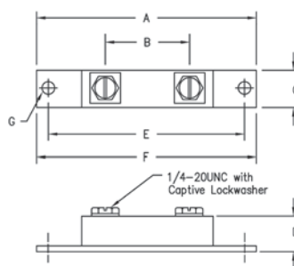
Twin Tower
