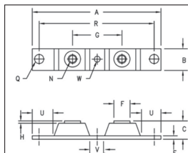
TO-244
