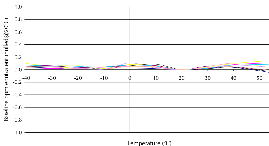
4CL Chlorine CiTiceL - Baseline vs Temperature
