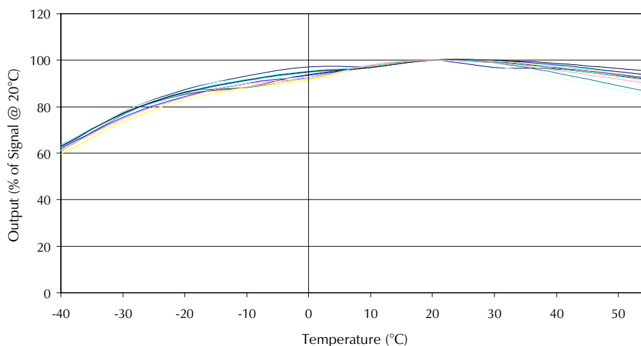
4CL Chlorine CiTiceL - Output vs Temperature
