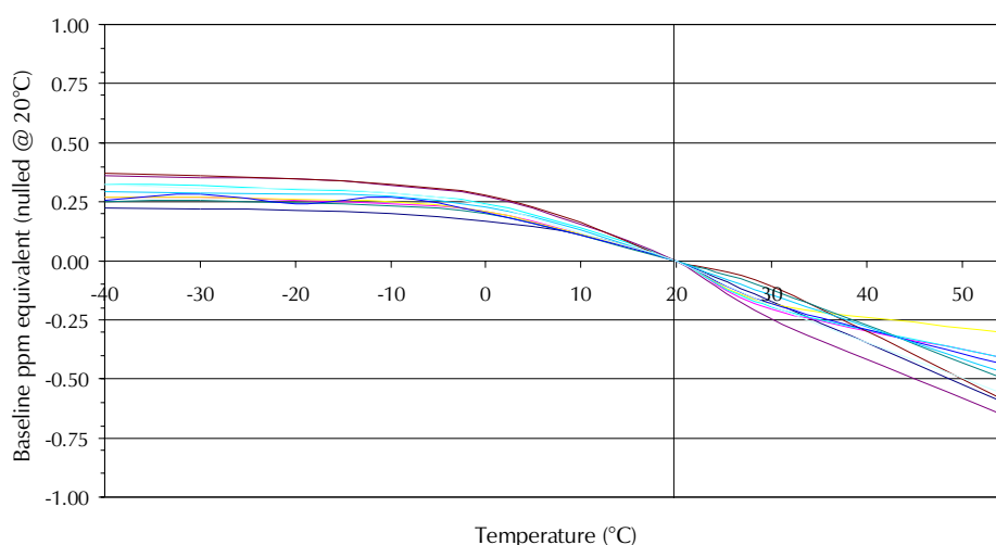
7CLH Chlorine CiTiceL - Baseline vs Temperature
