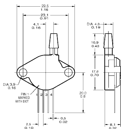
GT/AT Housing
