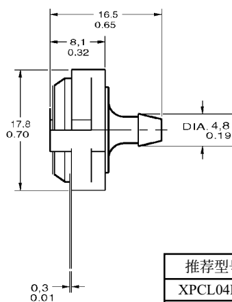
GBT Housing
