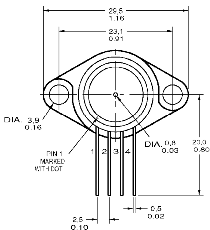
GBF Housing
