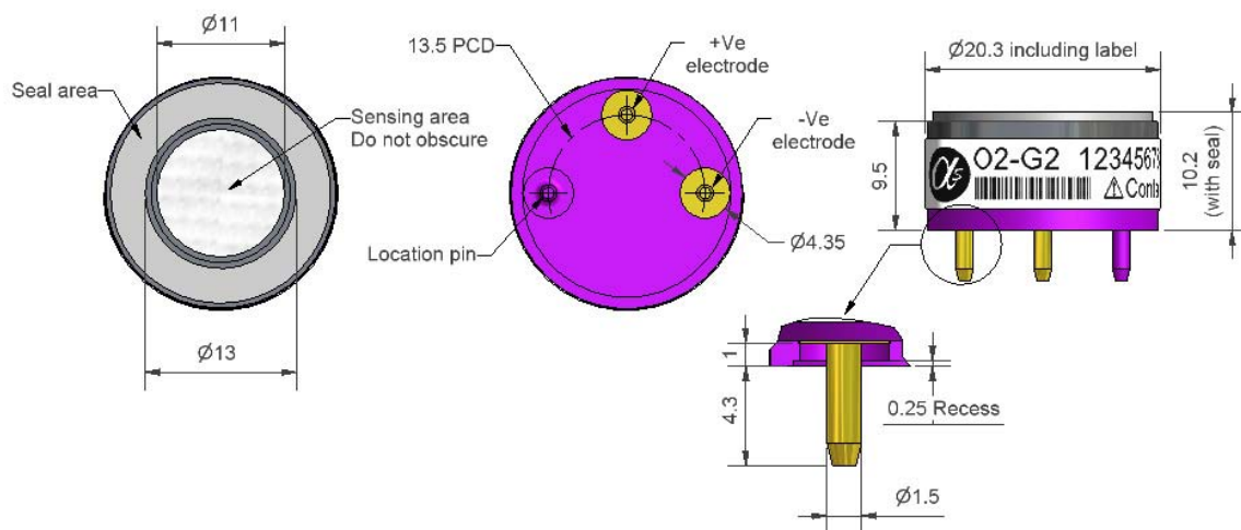
Figure 1 O2-G2 Schematic Diagram
