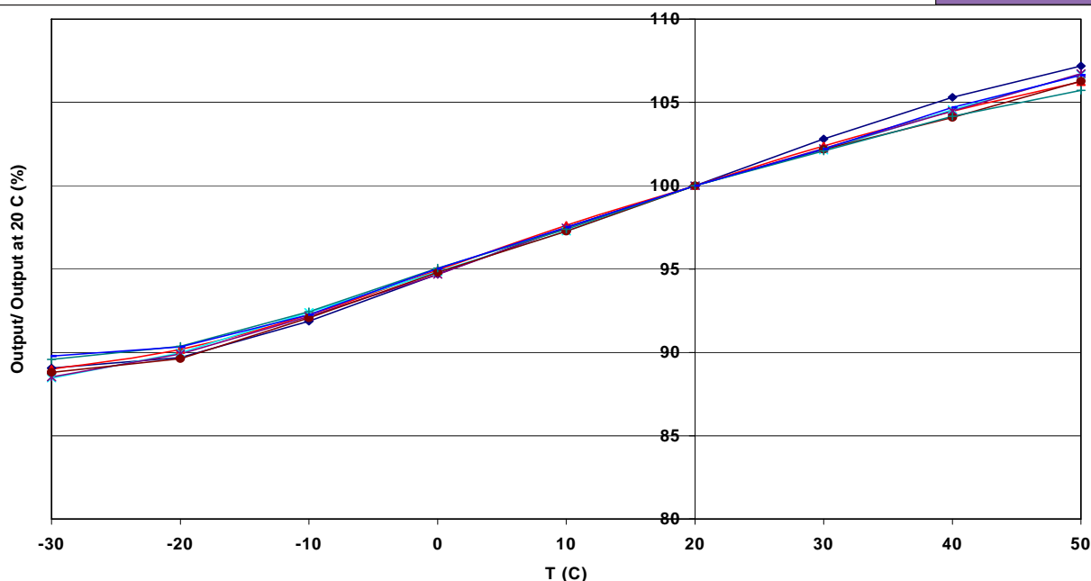
Figure 2 Temperature Performance
