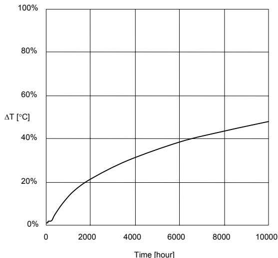
Fig. 5: Relative increase of R_h as a function of power-on time at ambient temperature
