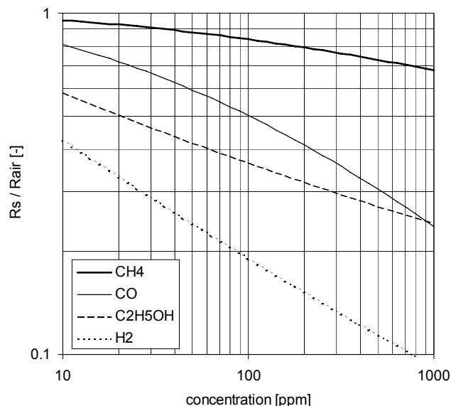
Fig. 6: Sensitivity to CO, H 2 , CH 4 , and C 2 H 5 OH at 25 °C and 50% RH
