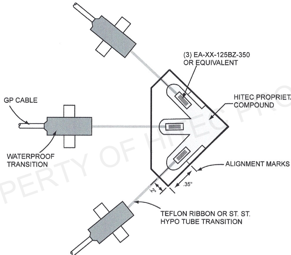
WIRING SCHEMATIC (X3)
