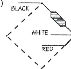
WIRING SCHEMATIC (X3)
