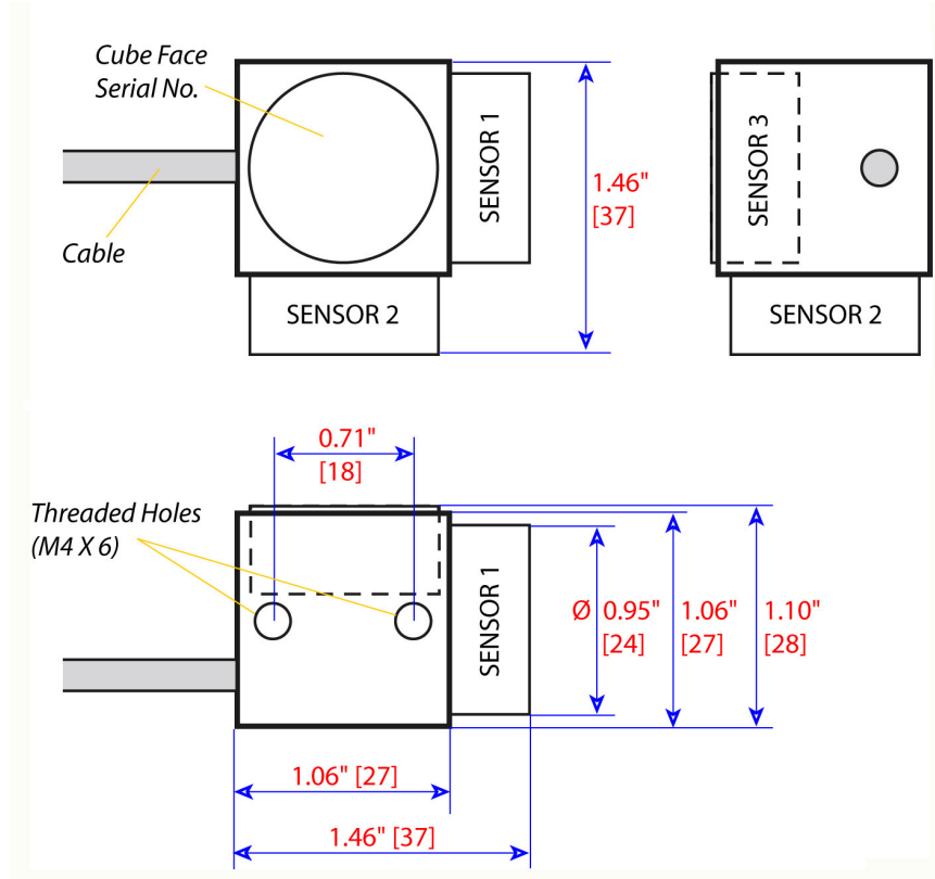
Figure 1: Dimensions (inches [mm])
