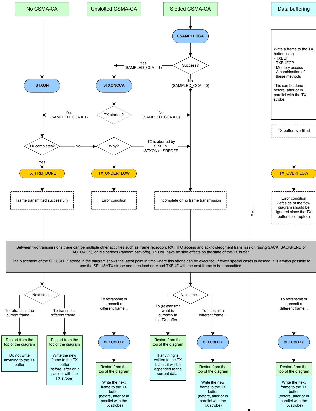
Figure 17: TX flow
