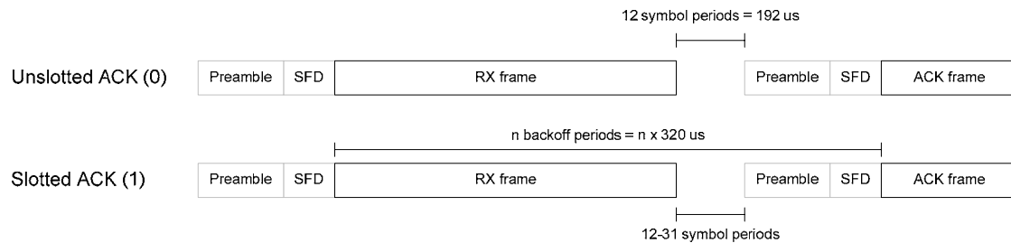
Figure 27: Acknowledgement timing
